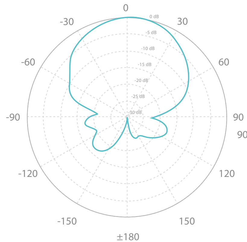
Horizontal Azimuth
