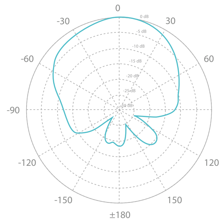
Horizontal Azimuth
