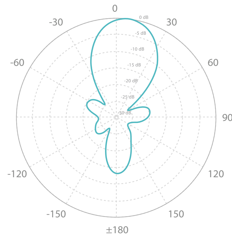
Horizontal Elevation
