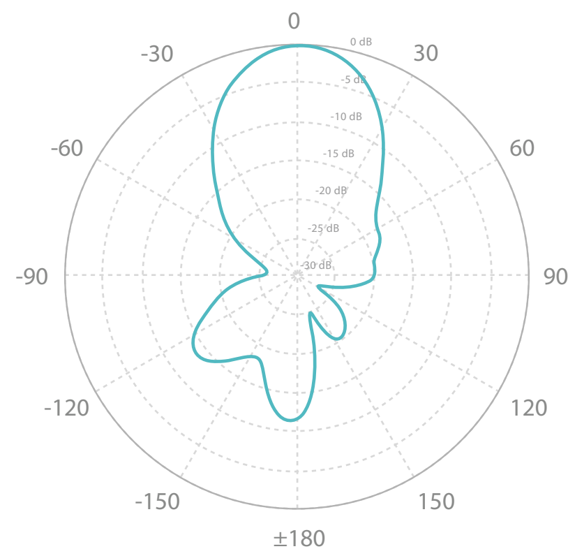
Vertical Elevation
