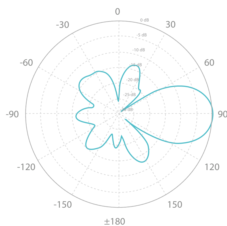
Horizontal Elevation
