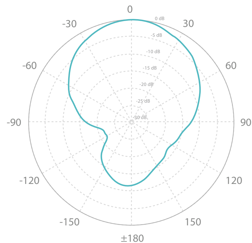
Vertical Azimuth
