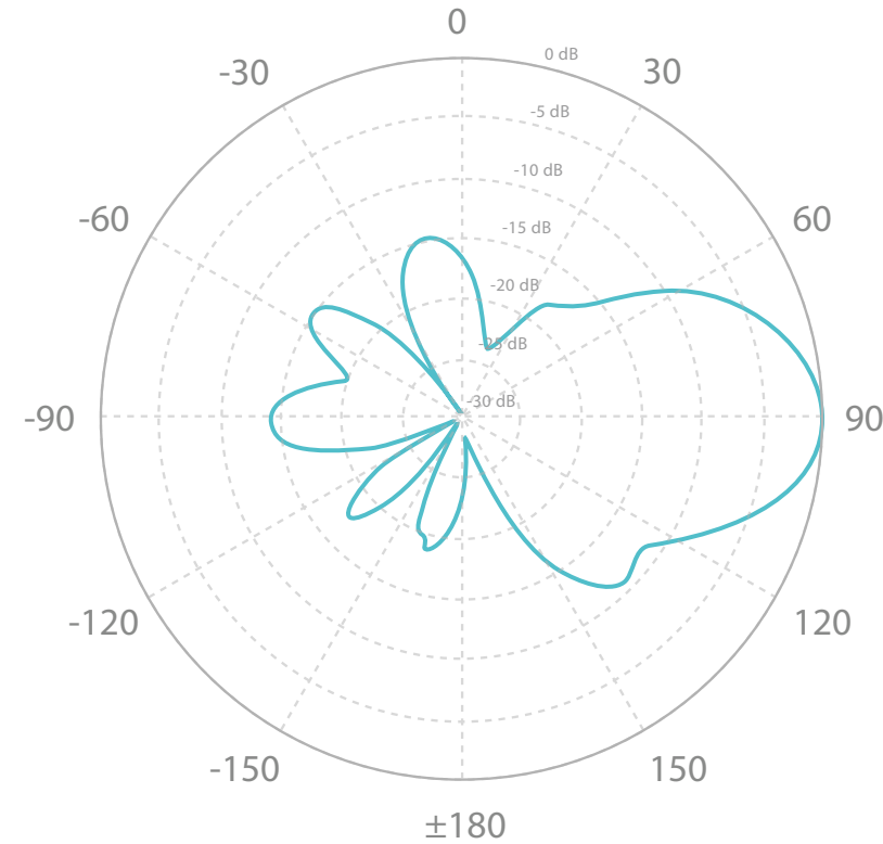
Horizontal Elevation
