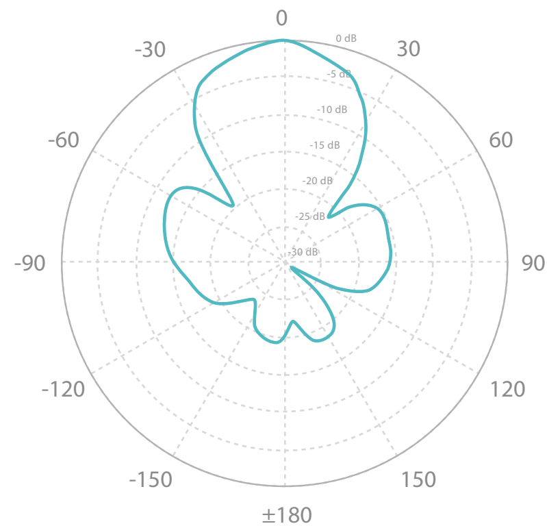
Horizontal Elevation
