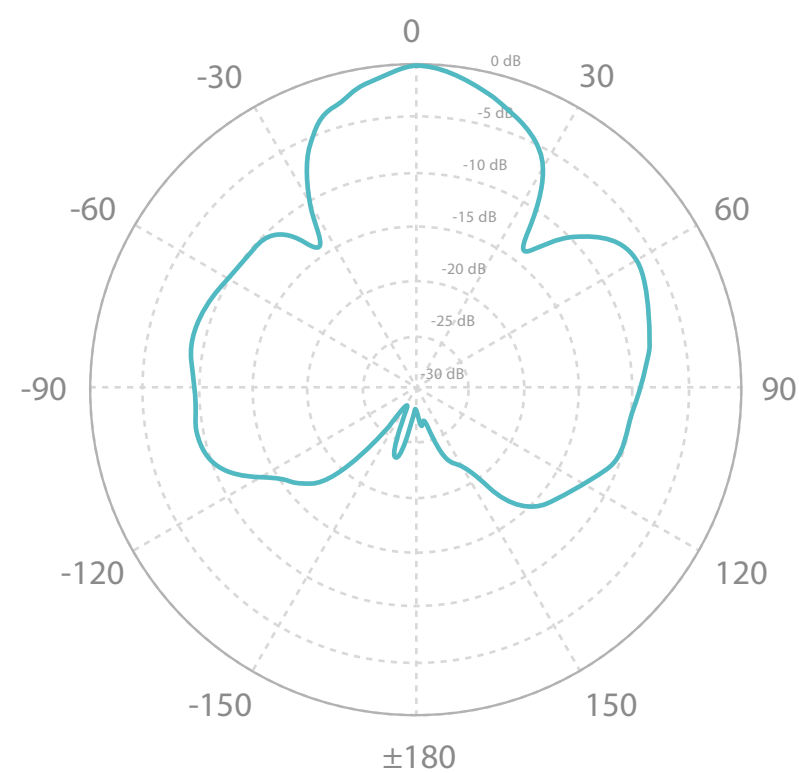
Horizontal Elevation
