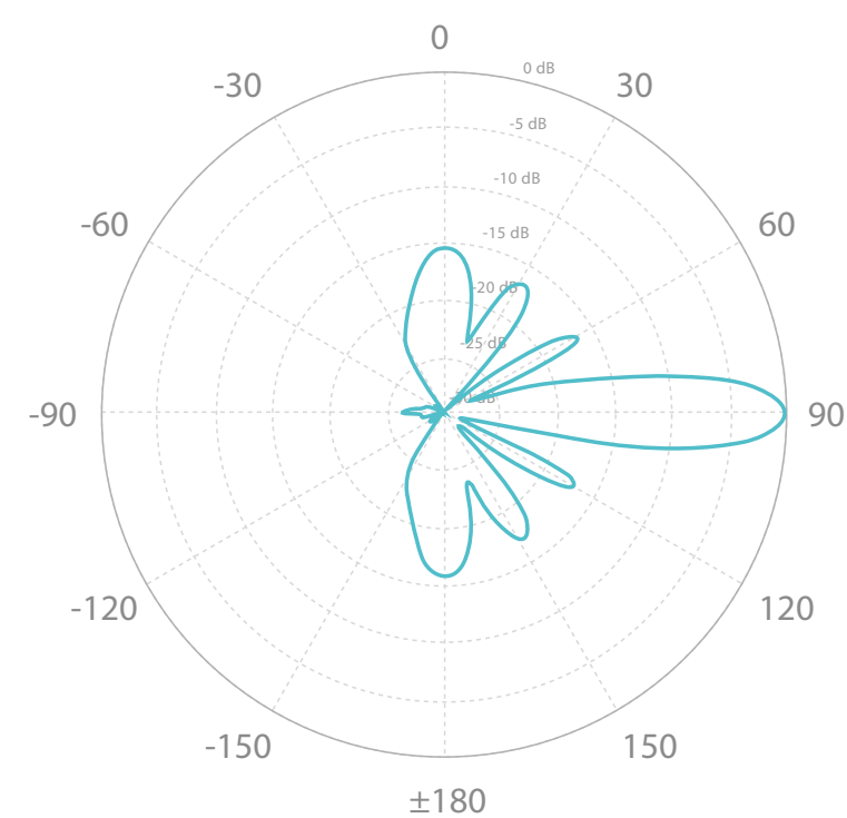
Horizontal Azimuth
