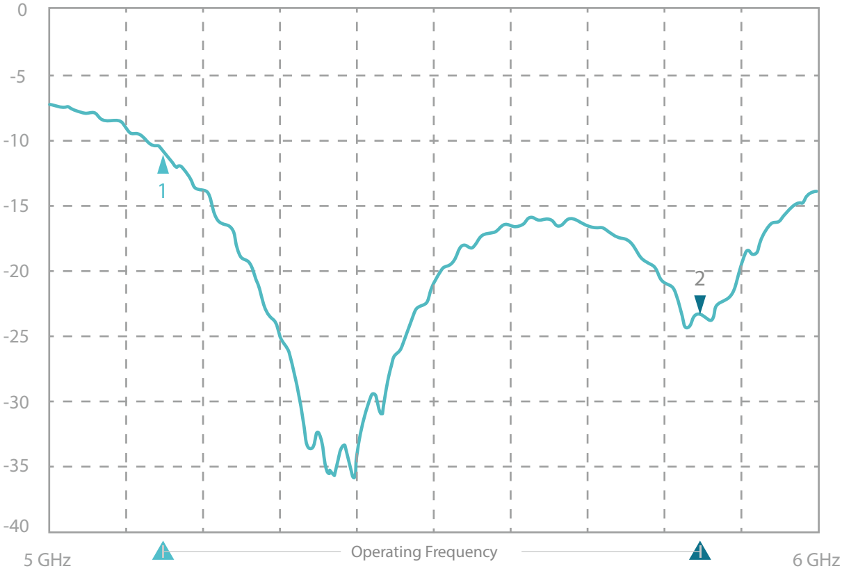
Return Loss
