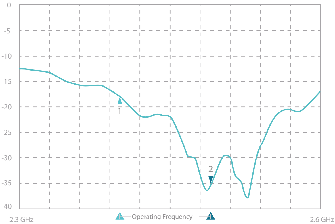
Return Loss – Horizontal Polarization
